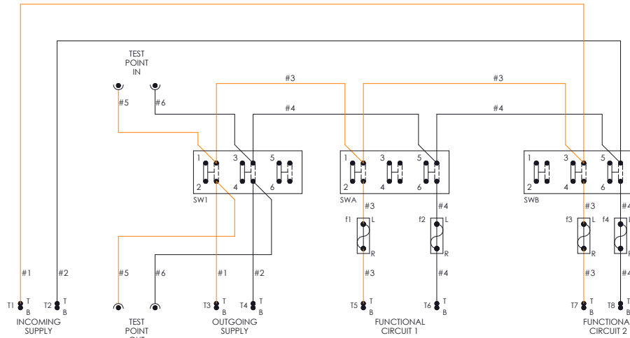
INTERNAL VIEW
