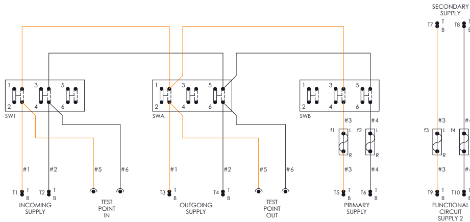
WIRING DIAGRAM
